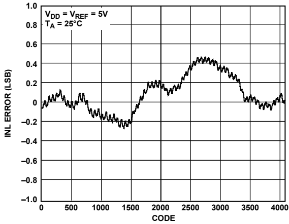
Figure 11. INL—12-Bit DAC
