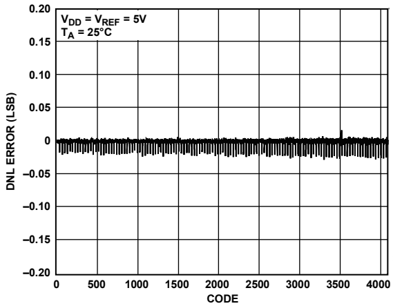
Figure 12. DNL—12-Bit DAC
