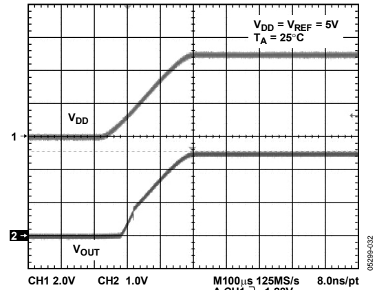
Figure 32. Power-On Reset to Midscale
